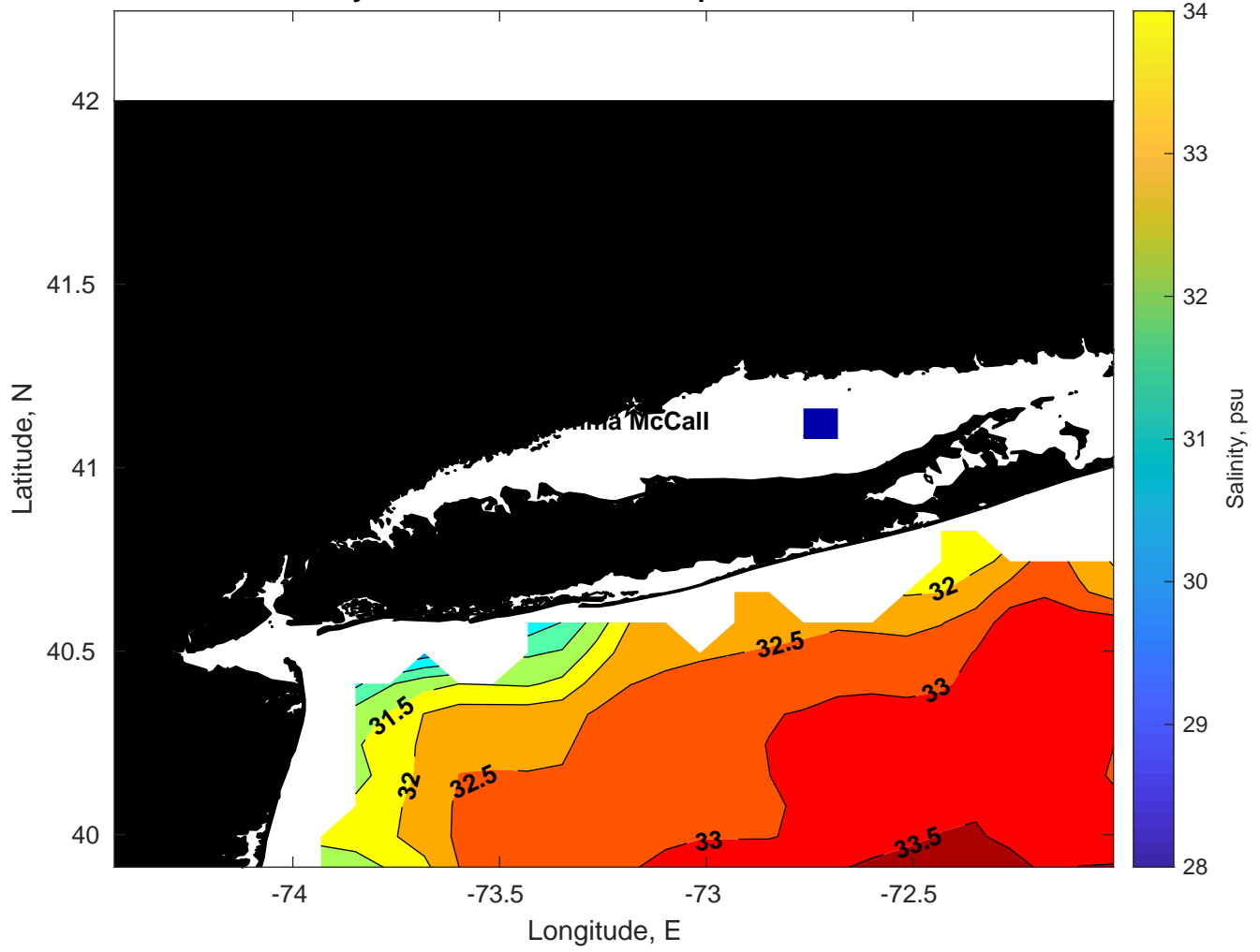
Surface Salinity for Emma McCall at 28-Apr-2024 00:00:00
